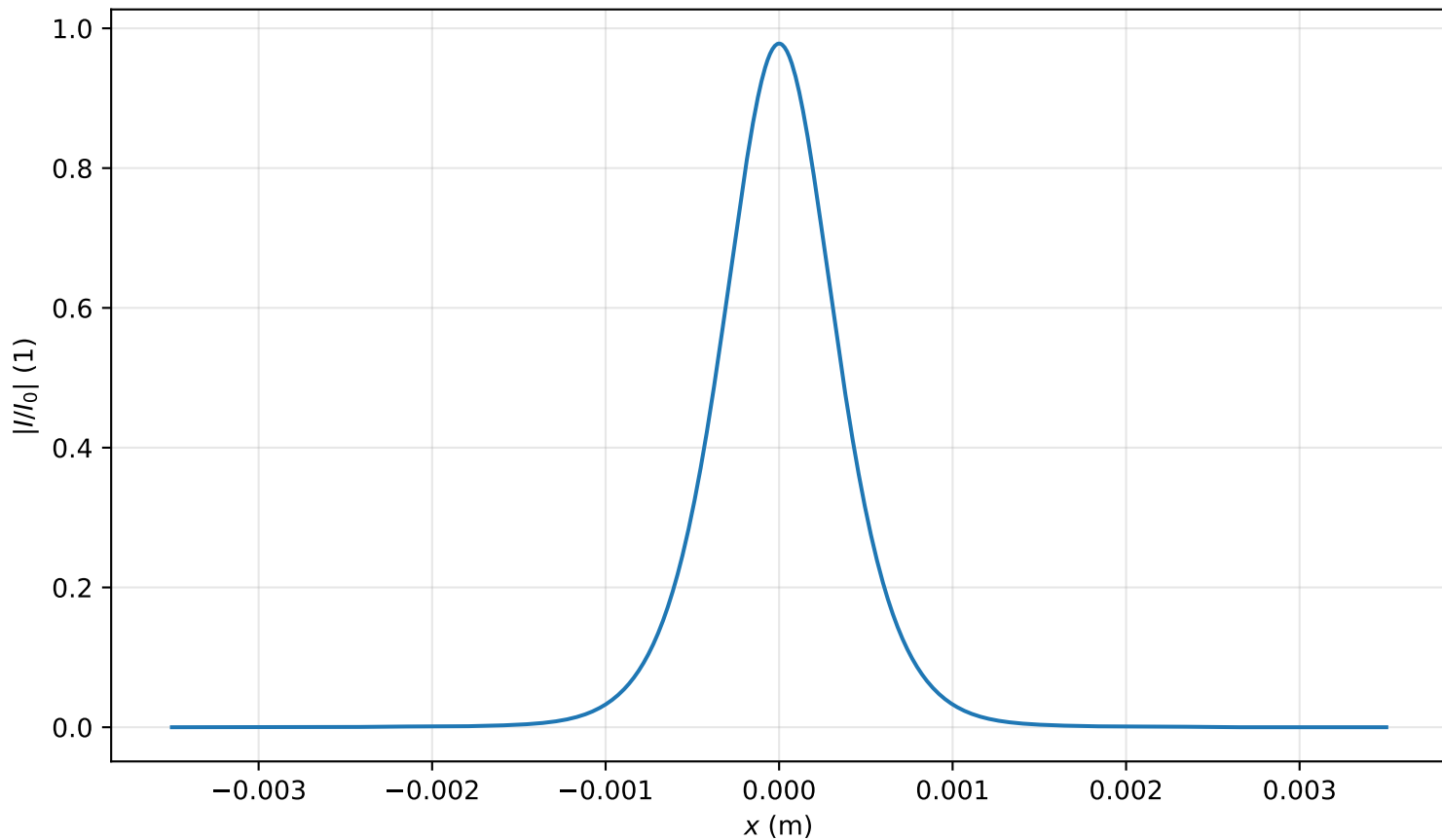
Intensity profile I(x, y = 0, z = 3.503m)/I_0 , P_{in}=0.8P_{cr} , artificial time
